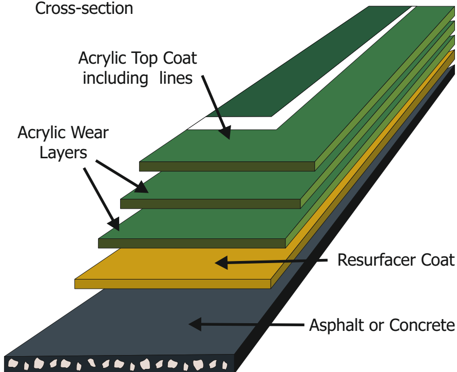
Sports-Cote™ Pro Hardcourt Cross-section
